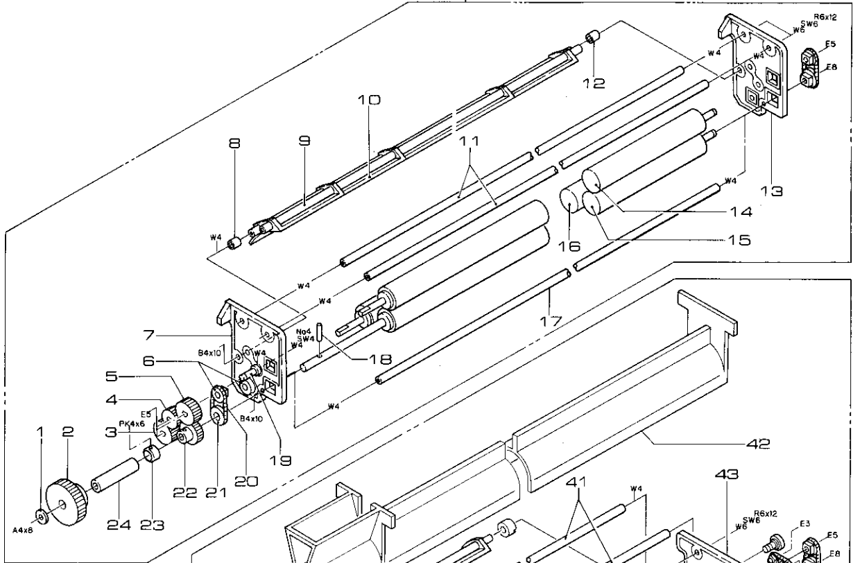
1 Entrance Rack
